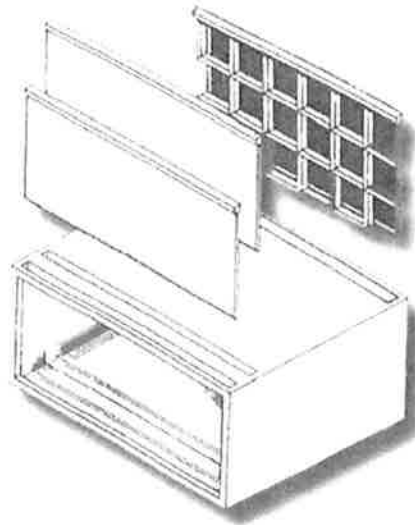
FIGURE 1—FLOOD FLAPS ® FLOOD VENT
